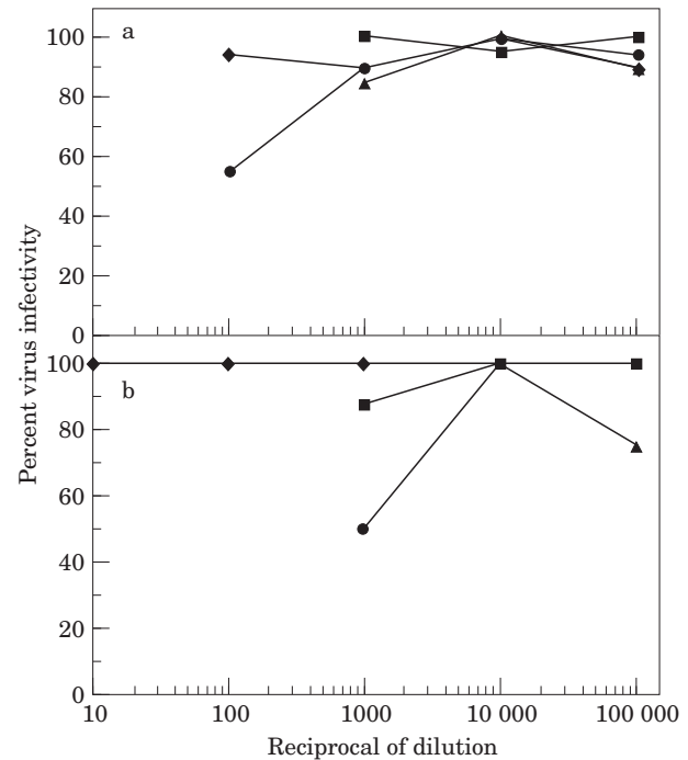
Figure 3 Infectivity of HCV-229E (a) and HCV-OC43 (b) after inactivation by chemical disinfectants: either 1.5% bleach (■), Proviiodine® (●), soap (▲) or 70% ethanol (◆). Only virus-disinfectants dilutions that were not cytotoxic in the infectious virus assay (see Table I) are shown. One hundred percent infectivity represents the infectious titre of virus incubated in PBS in the chemical disinfection assay.
